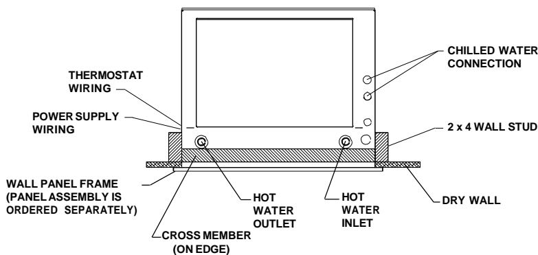
INSTALLED UNIT TOPVIEW Figure 2
